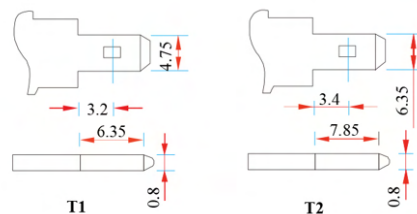
Terminal Dimensions
