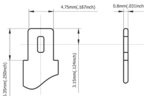
Terminal Dimensions
